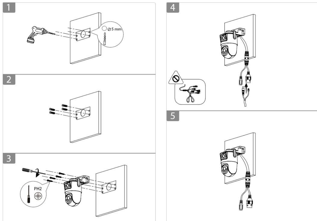
Figure 4-4 Wall mount
