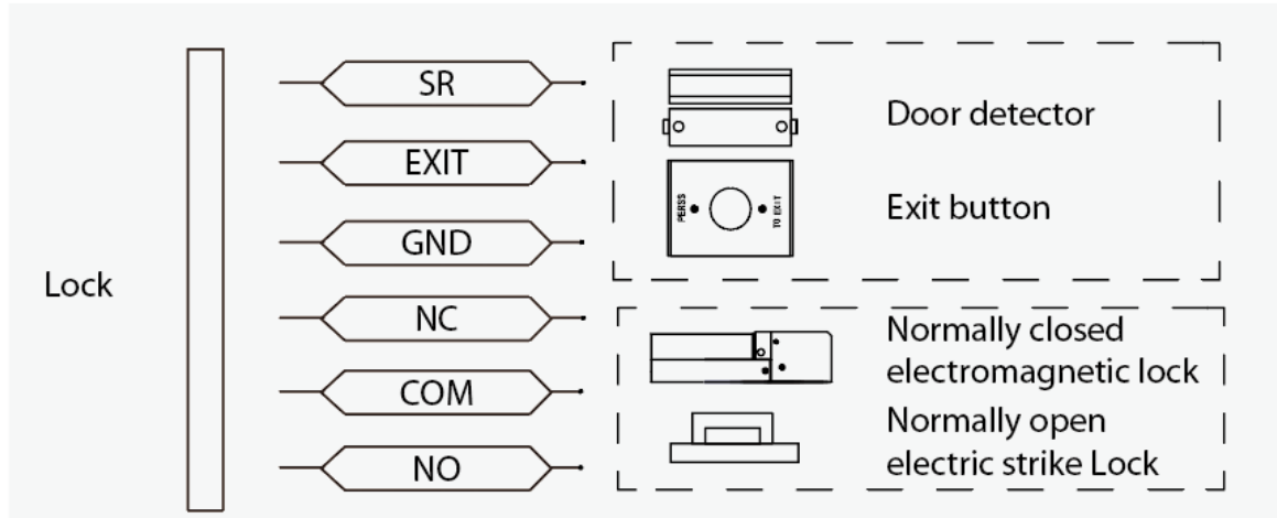
Figure 3-1 Wiring
