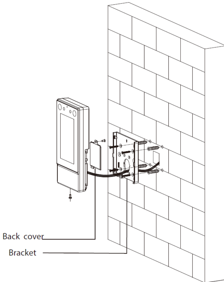
Figure 2-6 Wall mount
