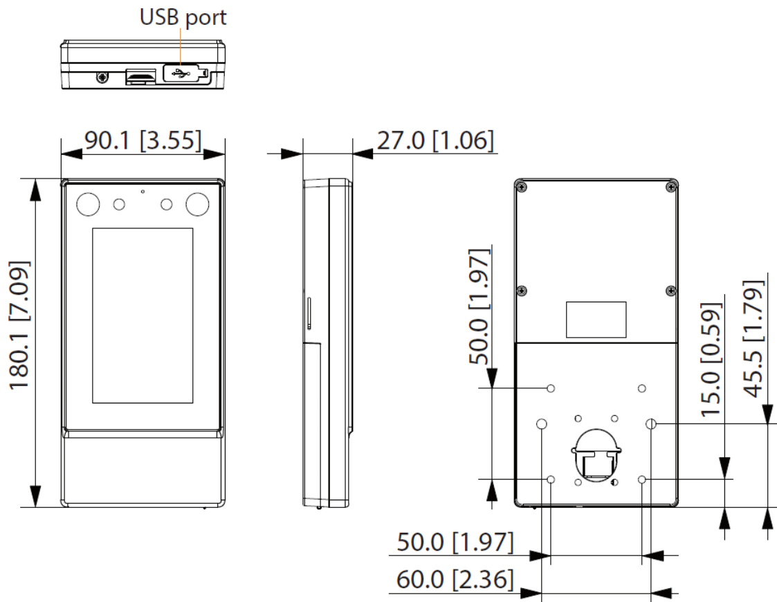
Figure 1-1 Appearance of Access Controller (Unit: mm [inch])
