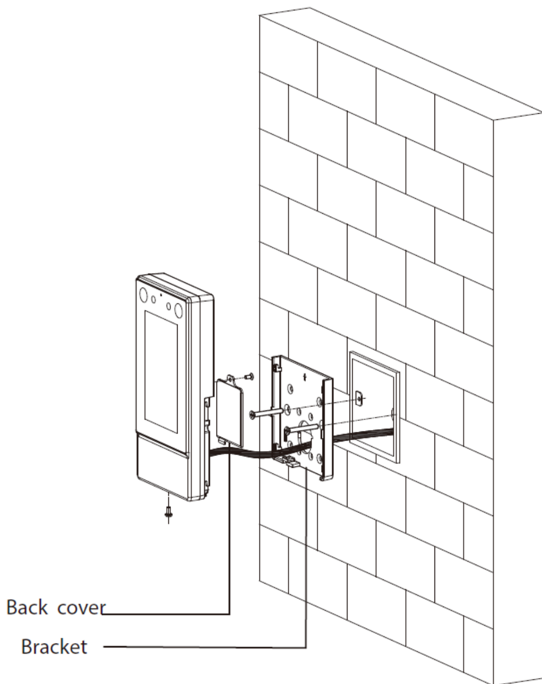
Figure 2-7 86 box mount
