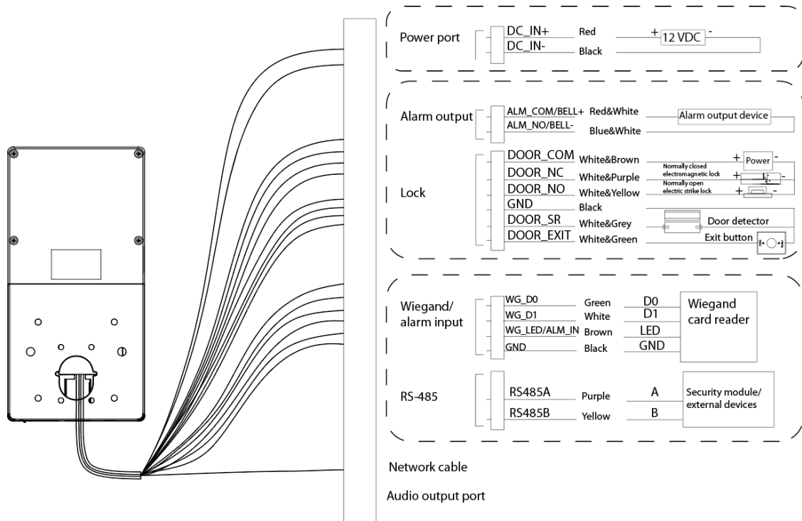
Figure 2-1 Wiring
