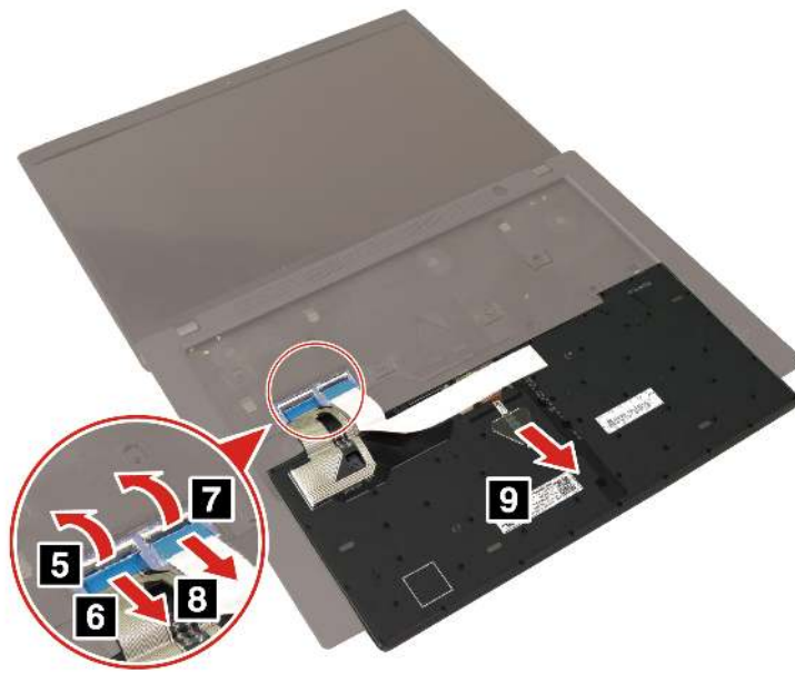
Removal steps of the keyboard (for L15 Gen 3)
