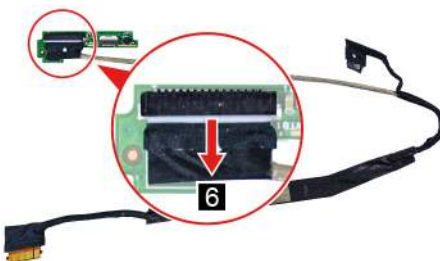
Figure 47. Disconnect the touch panel cable from the sensor board
