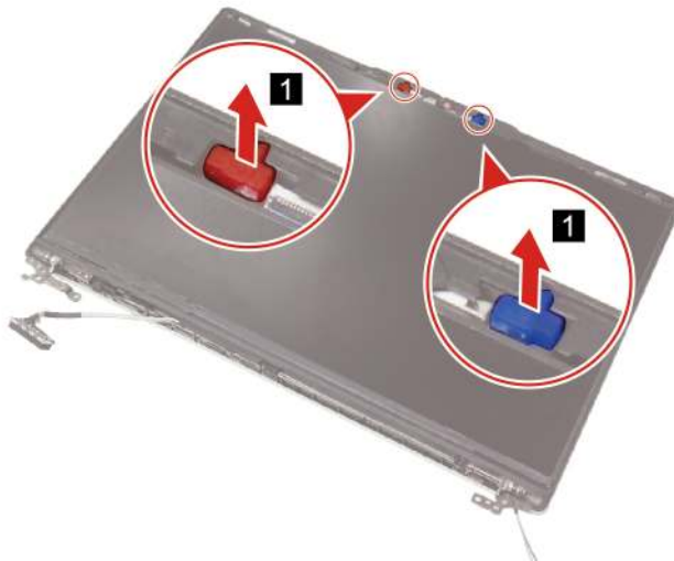
Figure 46. Remove the microphone rubbers
