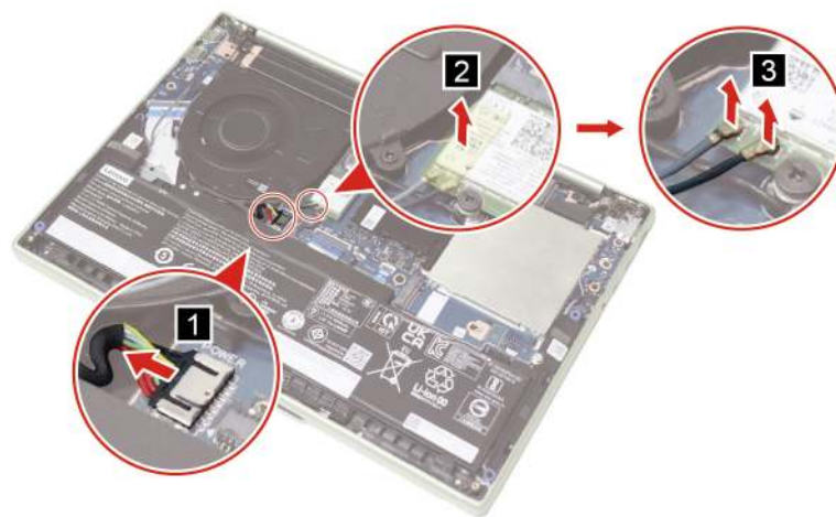
Figure 7. Disconnect the battery pack cable, remove the Wi-Fi card cover and disconnect the antennas
