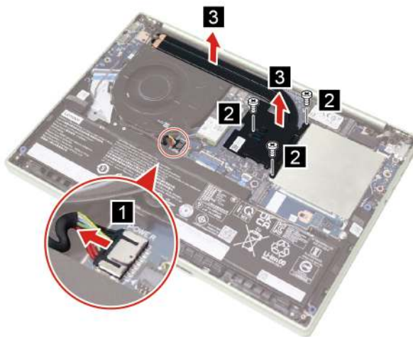
Figure 12. Disconnect the battery pack cable, remove three screws, and remove the heat sink
