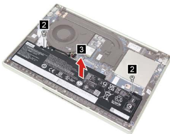
Figure 5. Remove two screws and remove the battery pack
