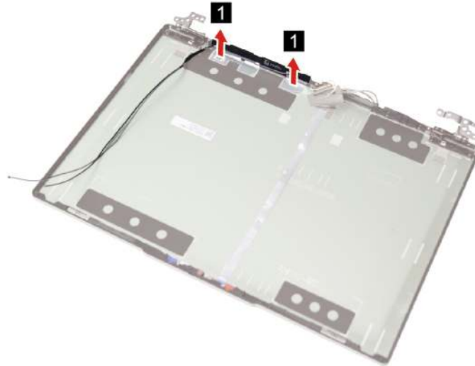
Figure 56. Remove the antennas
