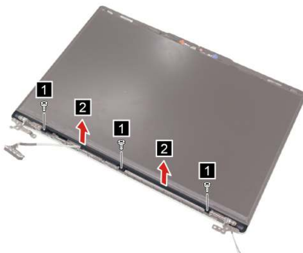
Figure 50. Remove three screws and the strip cover
