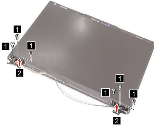
Figure 48. Remove six screws and the hinges
