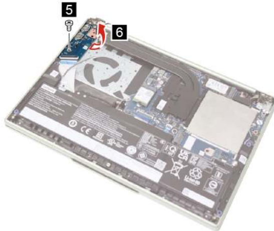
Figure 24. Remove one screw and the I/O board
