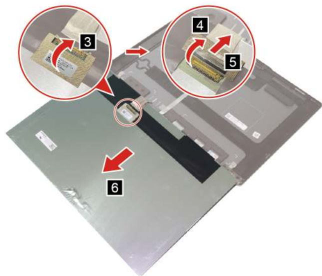
Figure 54. Disconnect the EDP cable and remove the OLED panel
