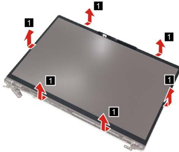
Figure 44. Remove the OLED/LCD bezel
