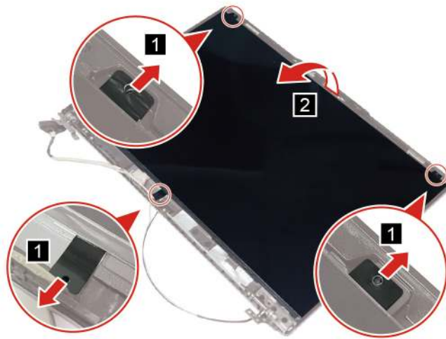
Figure 53. Pull out five pieces of the removable tape and turn over the OLED panel
