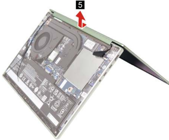
Figure 39. Rotate the OLED/LCD module and remove the OLED/LCD module
