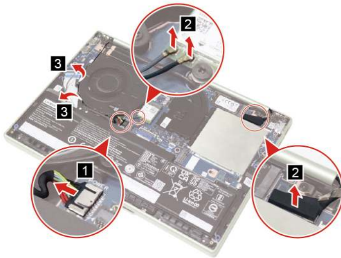
Figure 37. Disconnect the battery pack cable, EDP cable, and antennas
