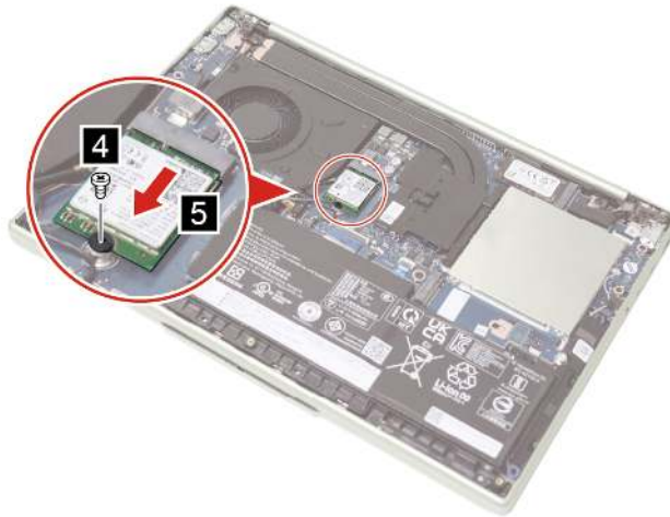
Figure 8. Remove one screw and the Wi-Fi card
