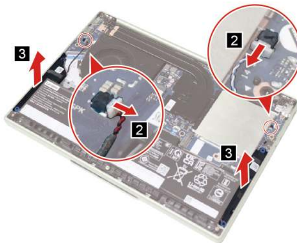
Figure 21. Disconnect and remove the speakers
