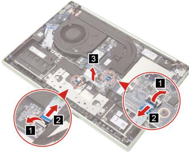
Figure 25. Disconnect and remove the touchpad cable
