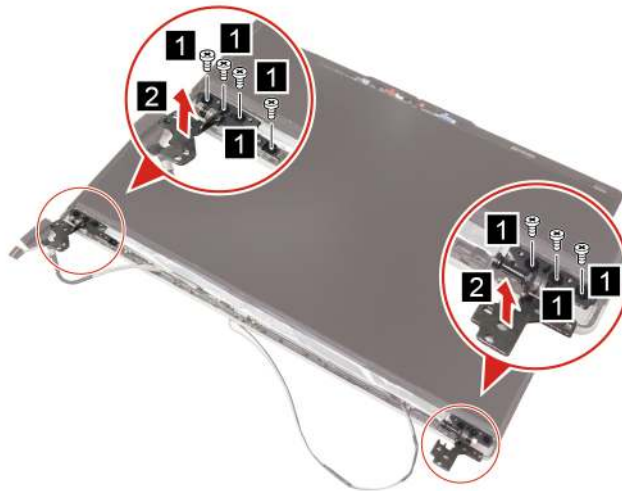
Figure 49. Remove seven screws and the hinges
