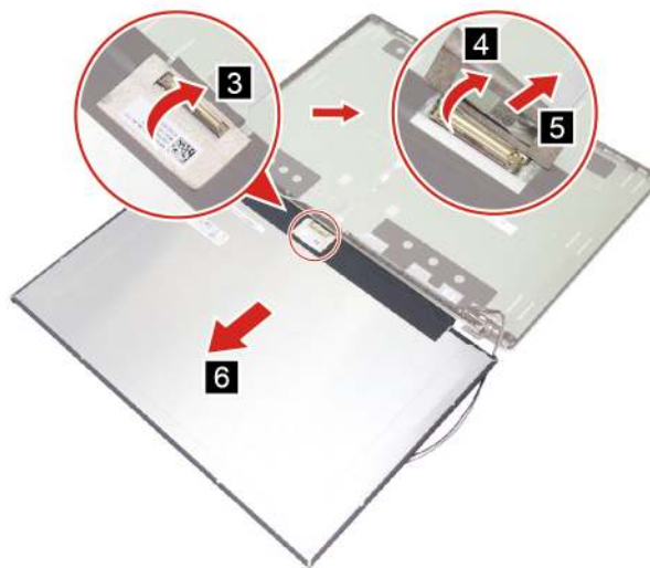
Figure 52. Disconnect the EDP cable and remove the LCD panel
