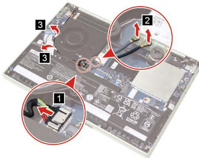
Figure 18. Disconnect the battery pack cable and antennas
