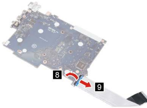
Figure 31. Disconnect and remove the I/O board cable
