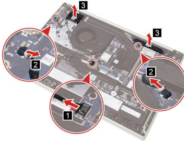
Figure 22. Disconnect and remove the speakers
