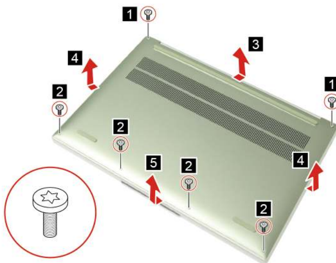
Figure 2. Remove six screws and the lower case
