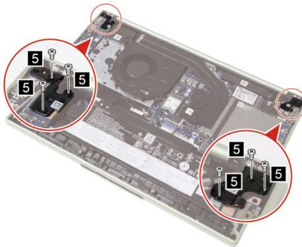
Figure 41. Remove six screws
