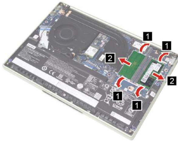
Figure 11. Open the latches and remove the memory module
