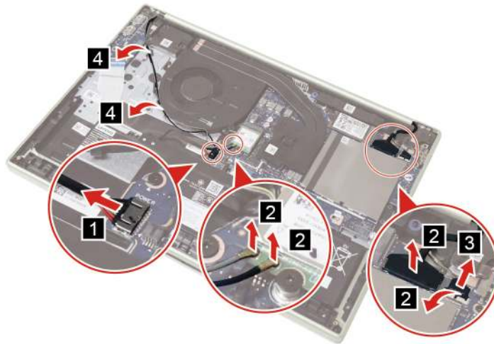
Figure 40. Disconnect the battery pack cable, EDP cable, and antennas
