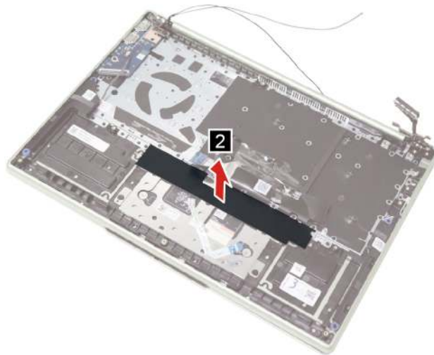
Figure 36. Remove the touchpad mylar
