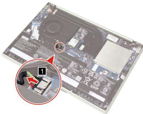
Figure 4. Disconnect the battery pack cable from the system board
