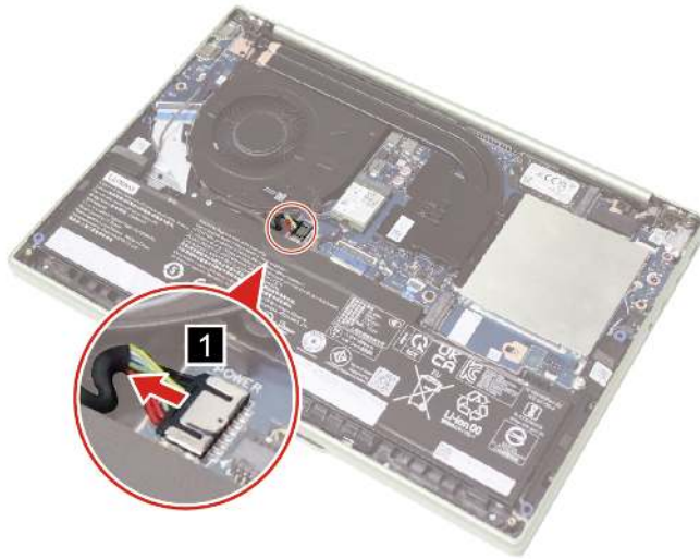
Figure 20. Disconnect the battery pack cable from the system board
