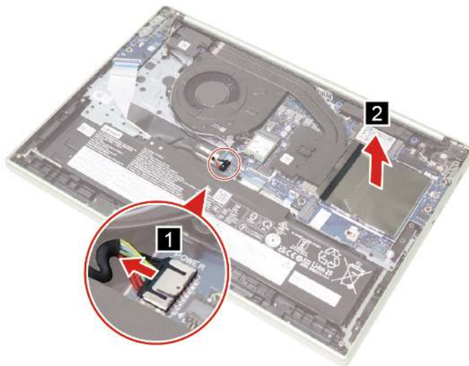
Figure 10. Disconnect the battery pack cable and remove the memory absorbing mylar
