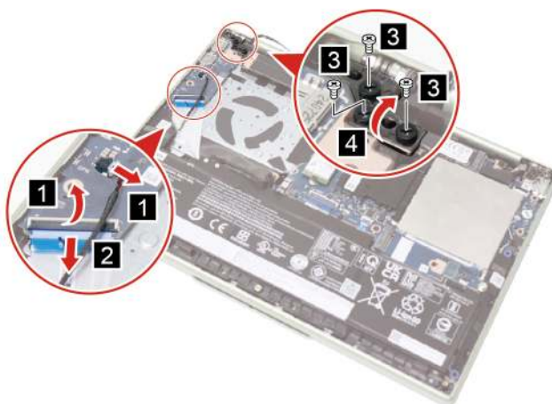
Figure 23. Disconnect the I/O board cable and left speaker cable, remove three screws, and open the left hinge
