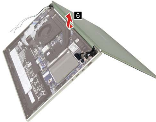
Figure 42. Rotate the OLED/LCD module and remove the OLED/LCD module
