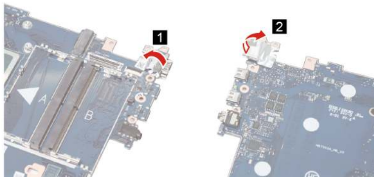
Figure 32. Remove the HDMI foil
