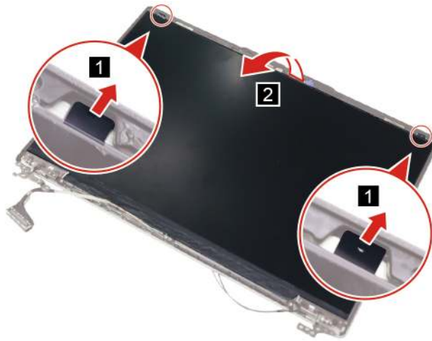
Figure 51. Pull out two pieces of the removable tape and turn over the LCD panel
