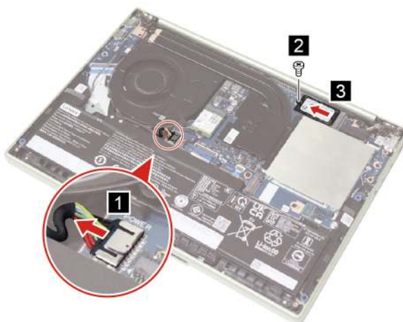
Figure 6. Disconnect the battery pack cable, remove one screw, and remove the M.2 solid-state drive
