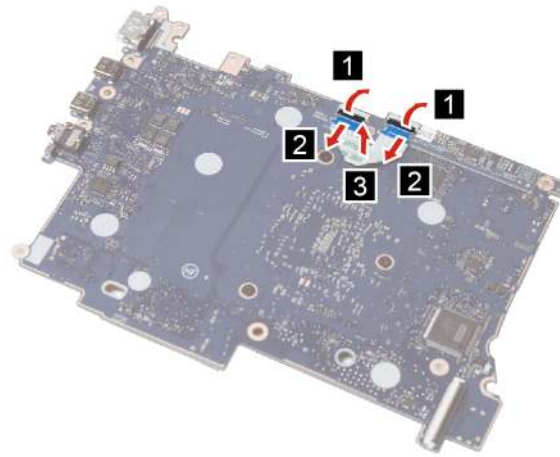
Figure 33. Disconnect and remove the PMIC board FPC
