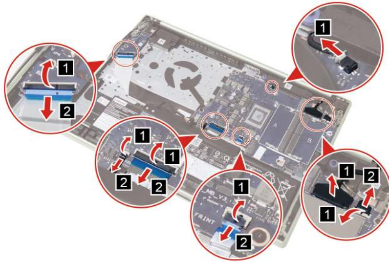
Figure 29. Disconnect cables
