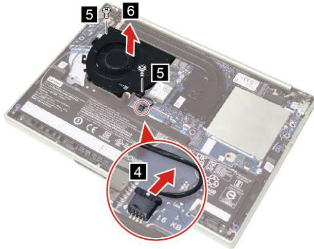
Figure 19. Disconnect the fan cable, remove two screws, and remove the fan
