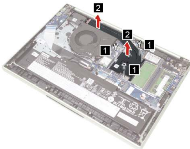
Figure 13. Remove three screws and the heat sink
