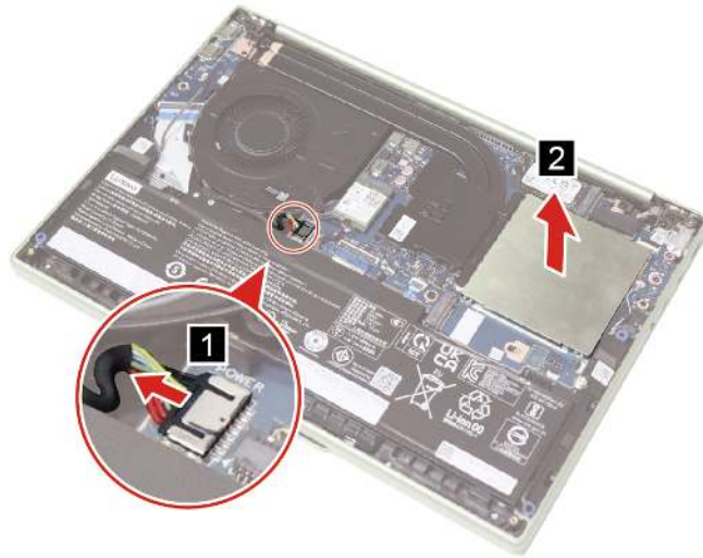
Figure 9. Disconnect the battery pack cable and remove the memory shield
