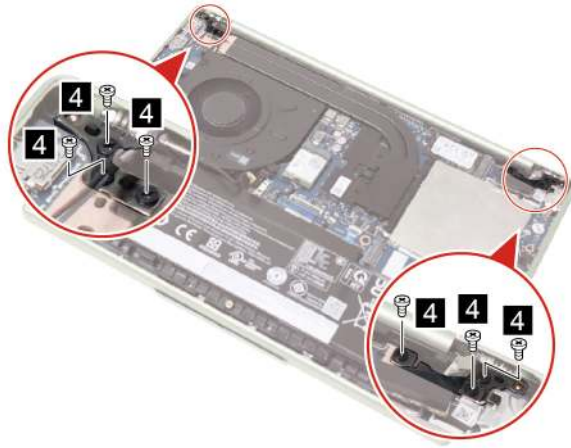
Figure 38. Remove six screws
