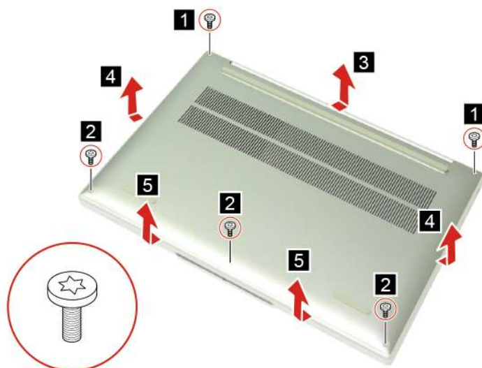
Figure 1. Remove five screws and the lower case
