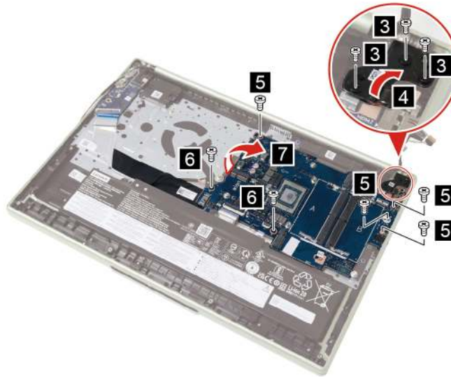
Figure 30. Remove eight screws and the system board
