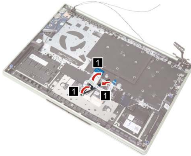
Figure 35. Peel back the cables
