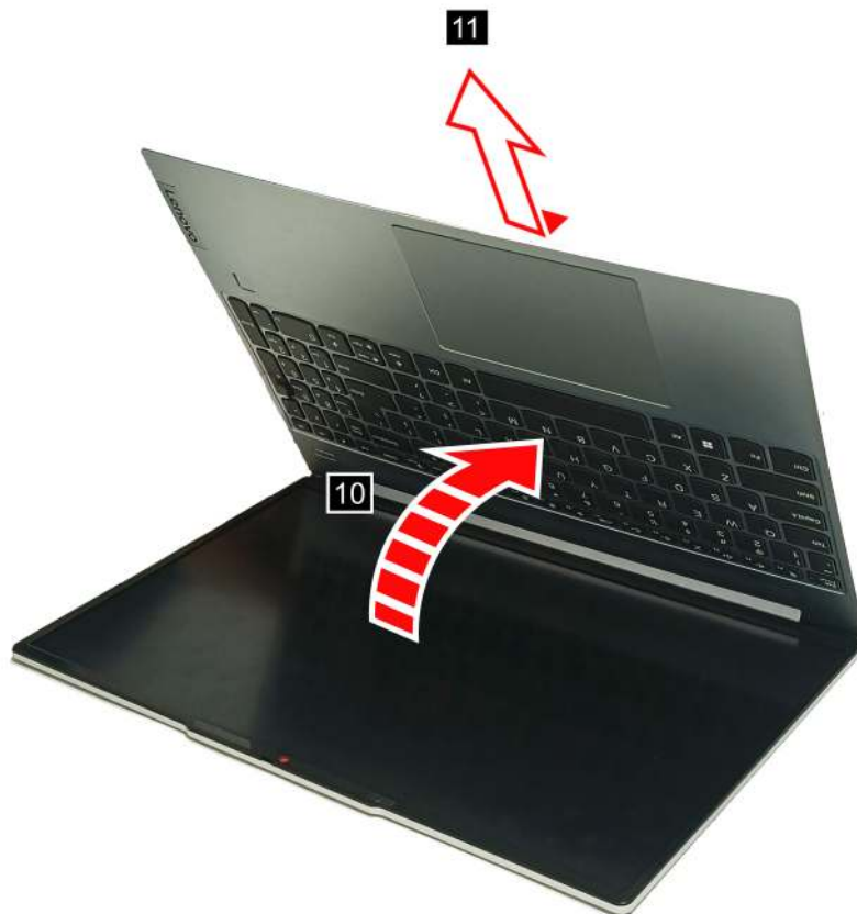
Figure 34. Remove the LCD unit
