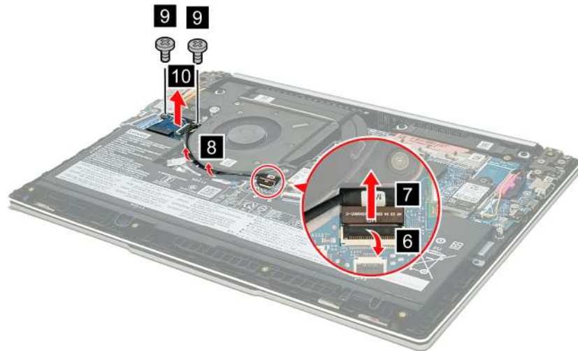
Figure 12. Remove the 2nd SSD module
