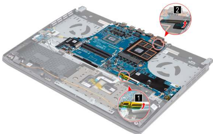
Figure 23. Remove the tape
