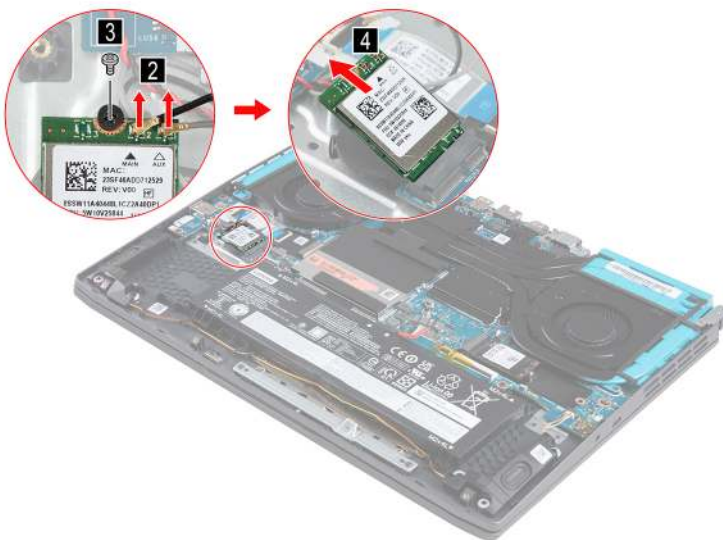
Figure 16. Remove the Wi-Fi card
