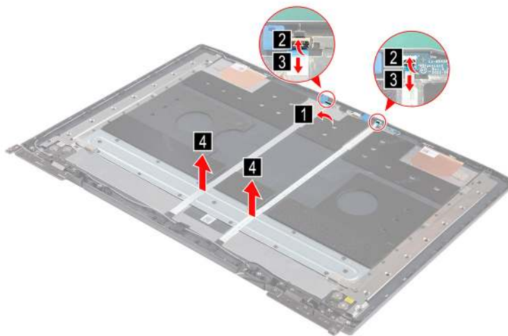
Figure 37. Remove the EDP cable
