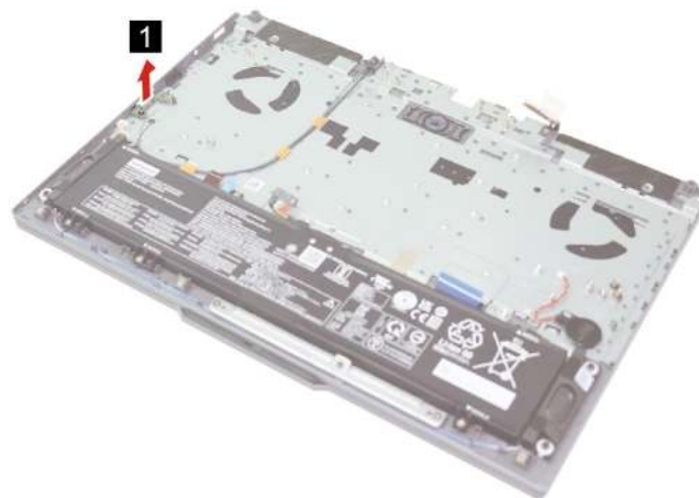
Figure 25. Remove the Type-C bracket
