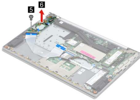
Figure 28. Remove the I/O board with cable
