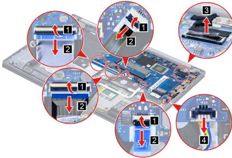
Figure 74. Disconnect cables
