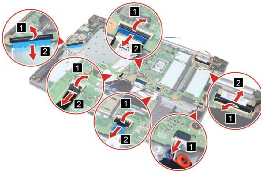
Figure 32. Disconnect cables
