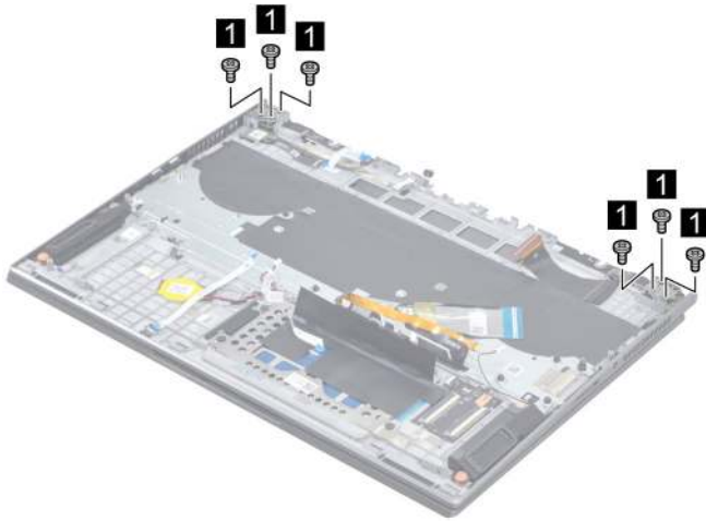
Figure 39. Remove six screws
