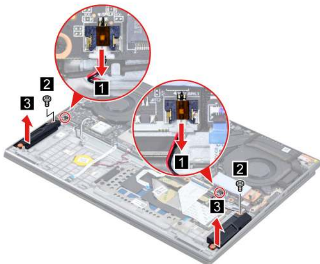
Figure 24. Remove the speakers
