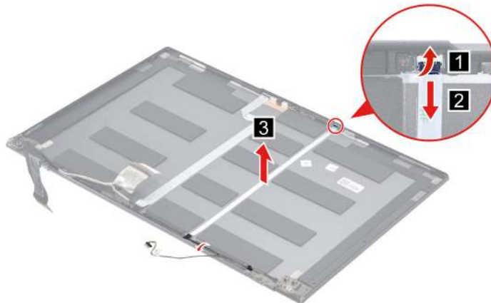
Figure 47. Remove the ambient light sensor (ALS) board cable
