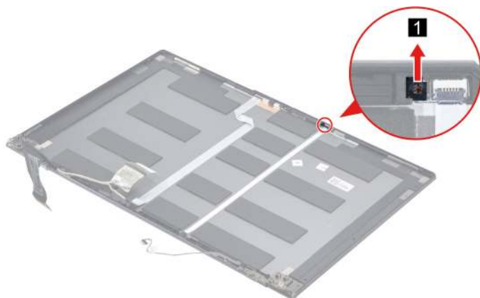
Figure 48. Remove the camera privacy shutter
