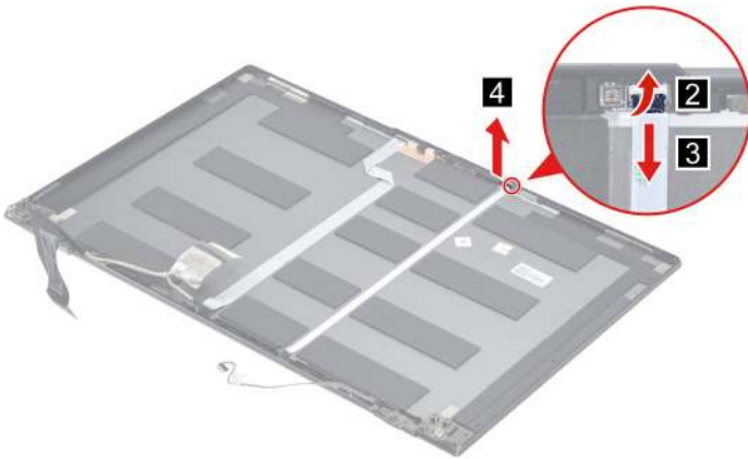
Figure 50. Remove the ambient light sensor (ALS) board
