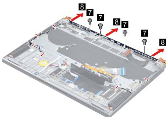
Figure 38. Remove the strip cover
