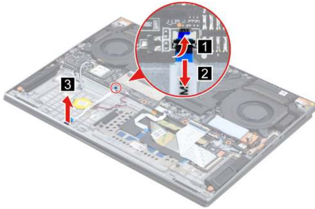
Figure 30. Disconnect the hall sensor board cable and remove the hall sensor board with cable
