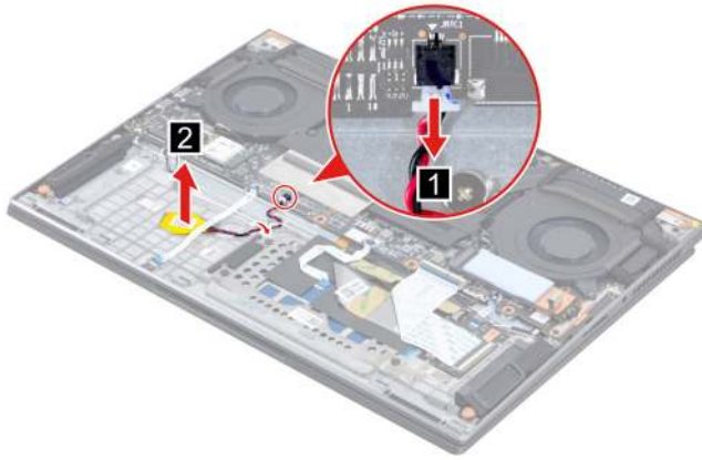
Figure 23. Disconnect the CMOS battery cable and remove the CMOS battery
