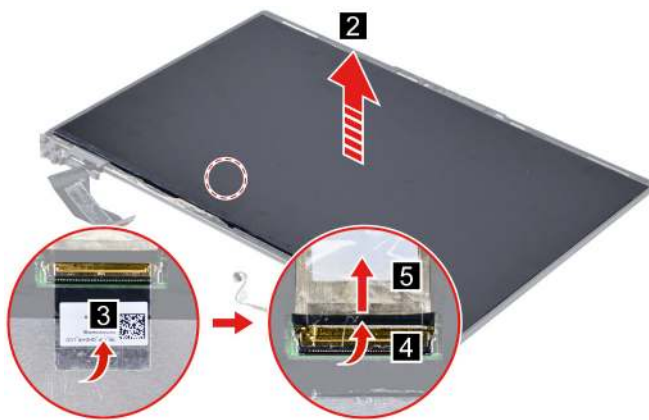
Figure 45. Disconnect the EDP cable and remove the LCD panel
