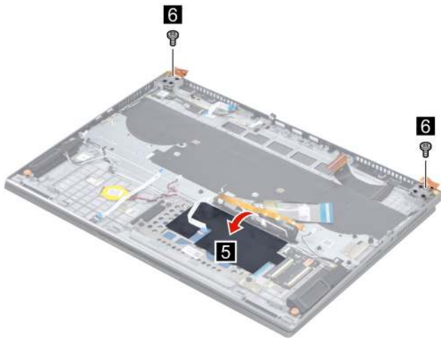
Figure 37. Peel back the touchpad board mylar
