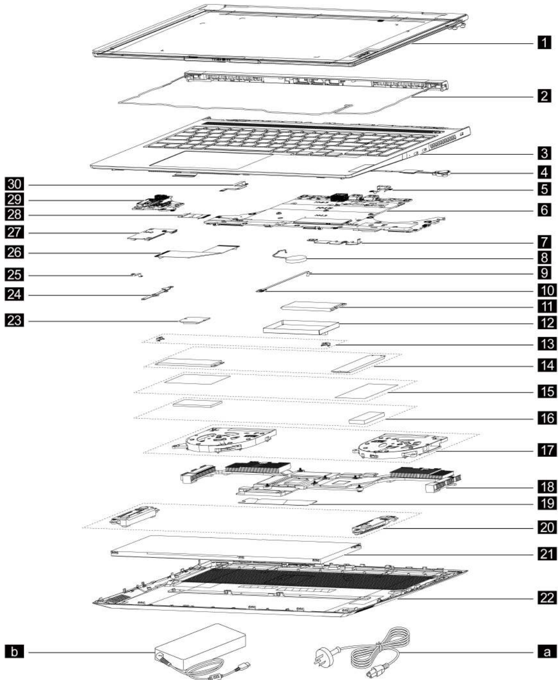
Figure 1. ThinkBook 16p G2 ACH exploded view
