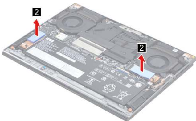
Figure 6. Remove the SSD Thermalpad
