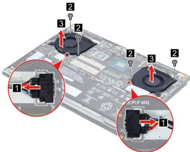
Figure 18. Remove the fans
