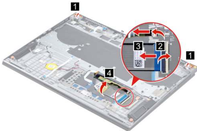
Figure 36. Remove the keyboard backlight cable
