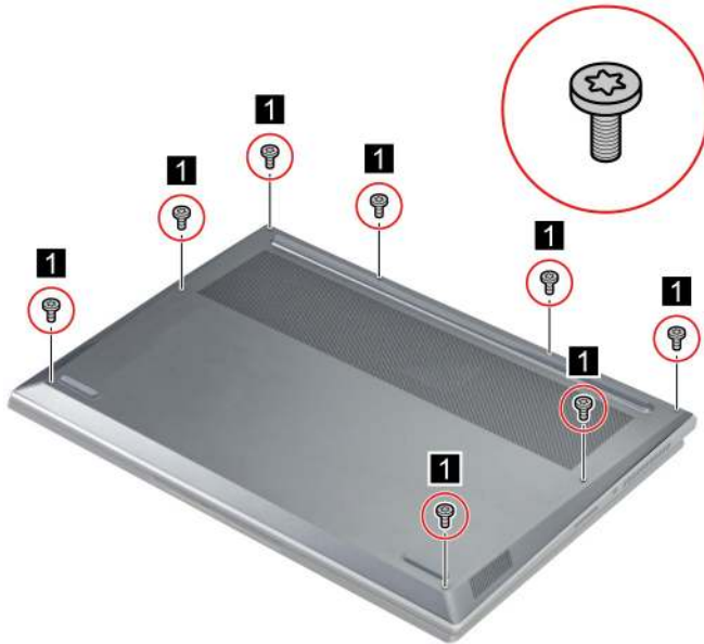
Figure 3. Remove eight screws
