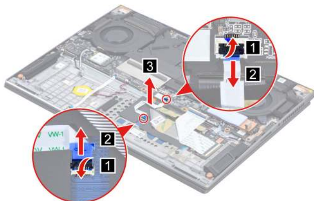
Figure 25. Remove the touchpad board cable
