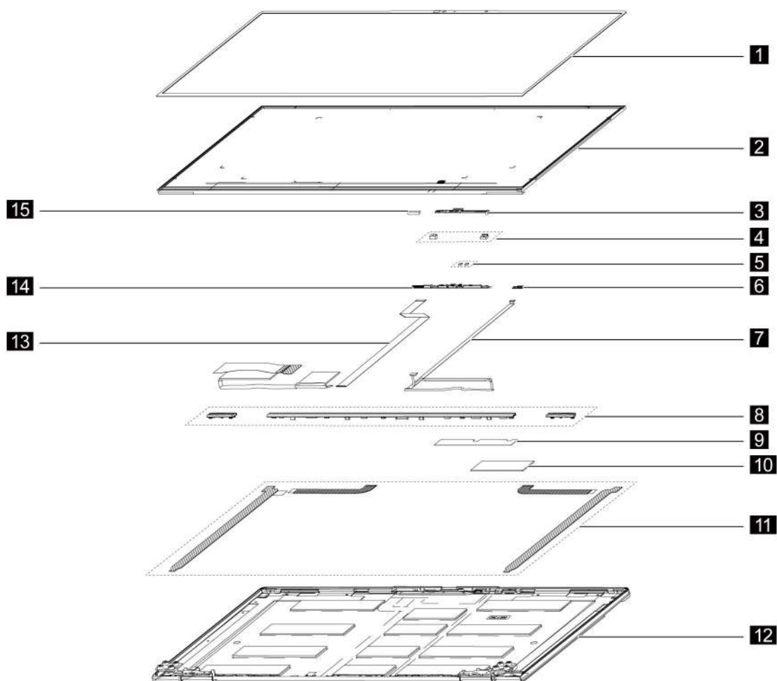
Figure 2. ThinkBook 16p G2 ACH LCD module — exploded view
