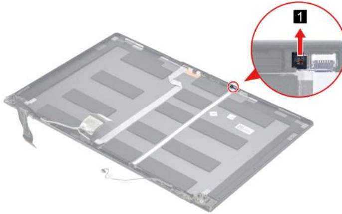
Figure 49. Remove the ambient light sensor (ALS) board rubber
