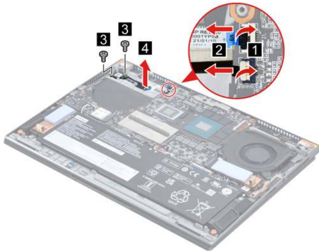
Figure 28. Disconnect the fingerprint board cable and remove the fingerprint board with cable
