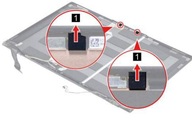
Figure 51. Remove the microphone rubbers
