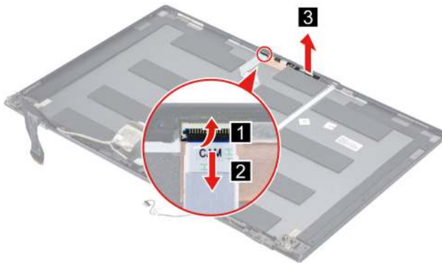
Figure 53. Remove the camera
