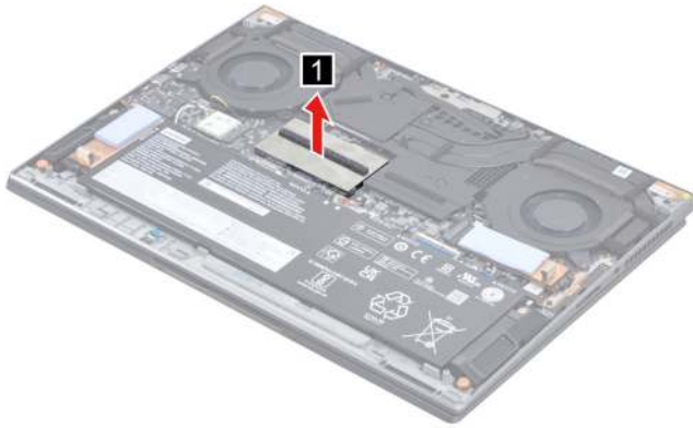
Figure 15. Remove the memory module shielding
