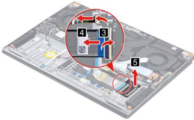
Figure 34. Remove the keyboard backlight cable
