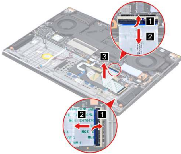
Figure 32. Remove the keyboard cable
