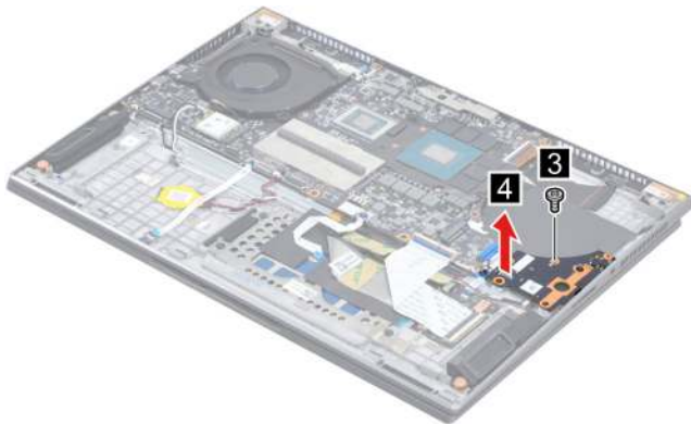
Figure 21. Remove the USB board with cable
