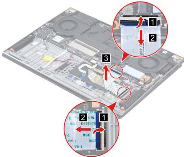
Figure 33. Disconnect the keyboard cable and keyboard backlight cable
