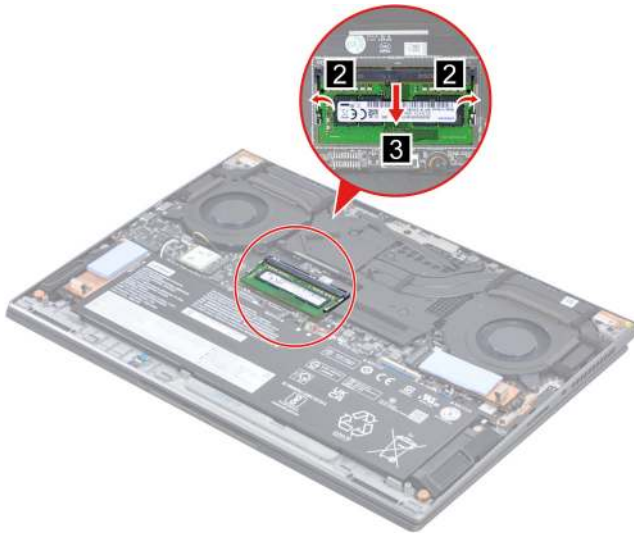
Figure 16. Remove the memory module
