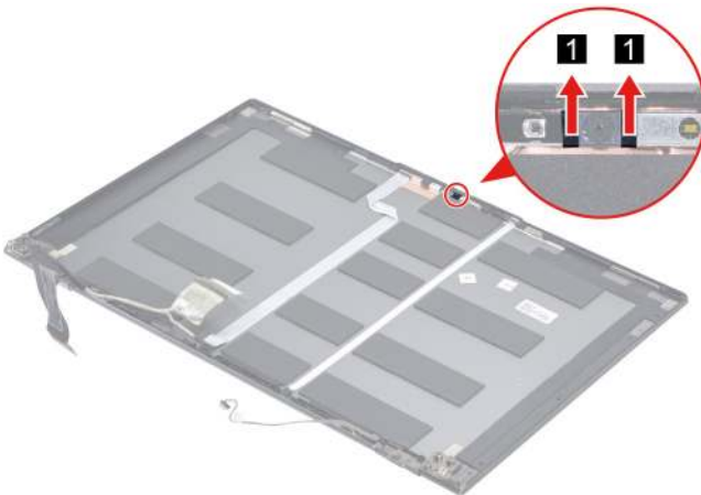
Figure 52. Remove the camera sponges
