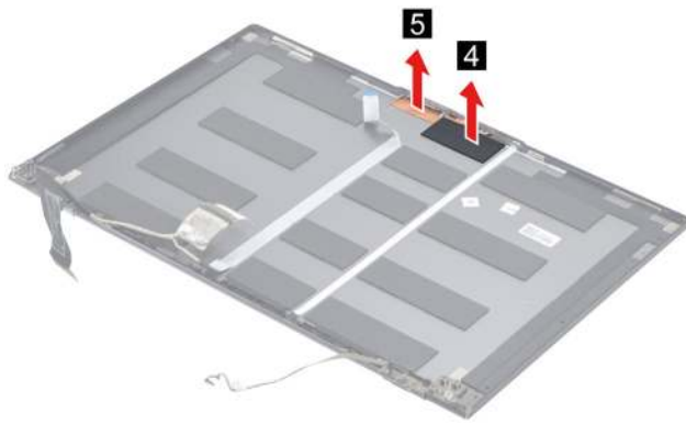
Figure 54. Remove the LCD sponge and then remove the foil
