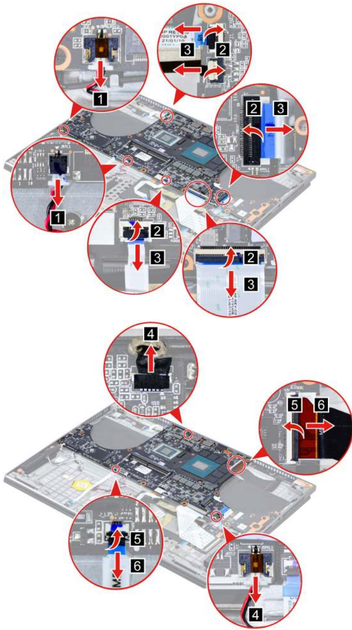
Figure 26. Disconnect cables
