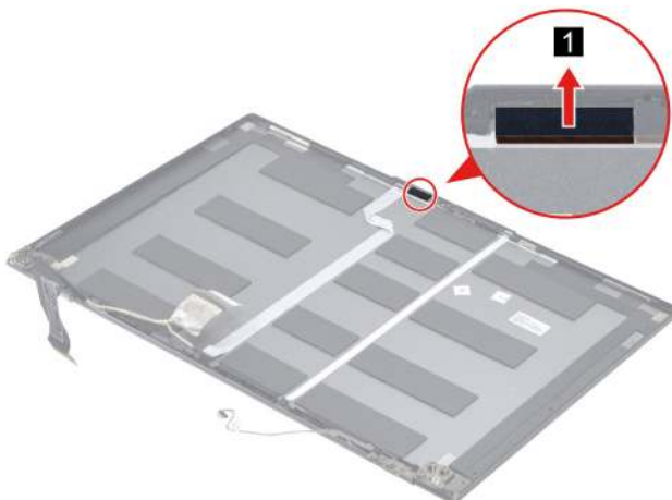
Figure 55. Remove the camera rubber
