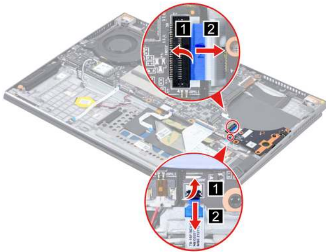
Figure 20. Disconnect the cable connected to the USB board and disconnect the USB board cable from the system board
