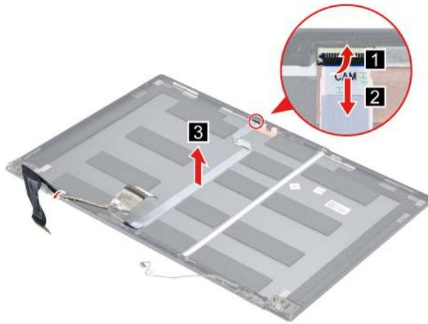
Figure 46. Remove the EDP cable
