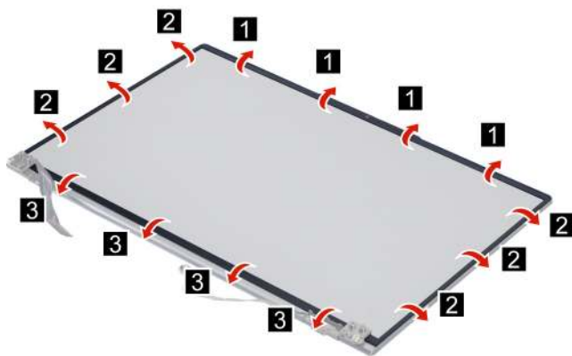
Figure 42. Remove the LCD bezel
