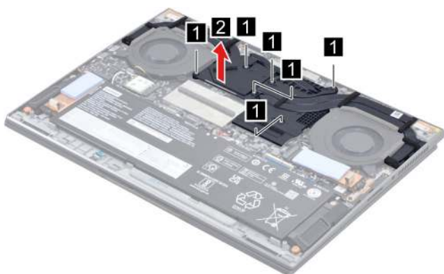
Figure 17. Loosen six screws and then remove the heat sink.
