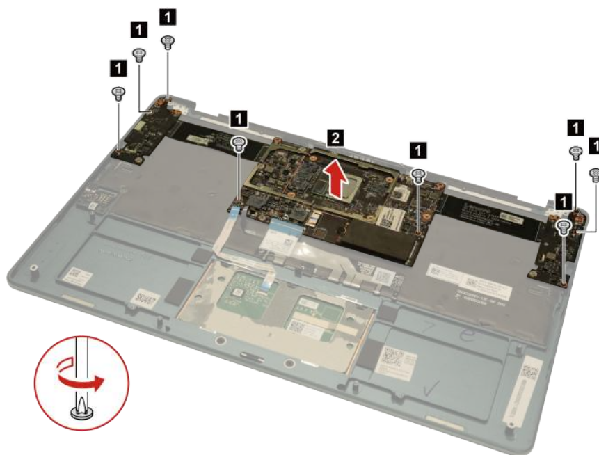
Figure 18. Remove the system board with I/O boards and I/O board cables
