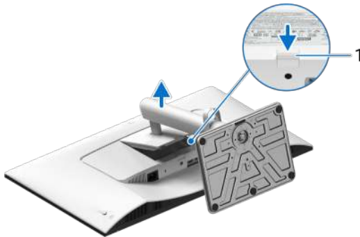
Figure 23. Removing the monitor stand
