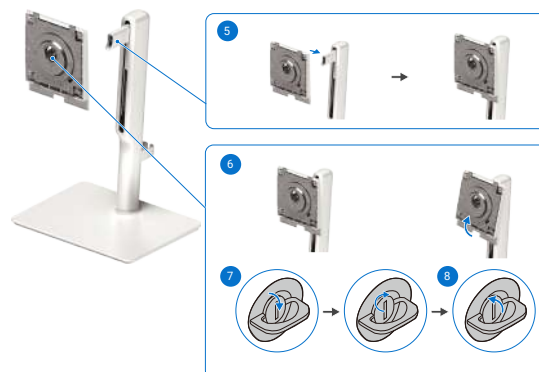
Figure 13. Install the VESA cover and stand riser
