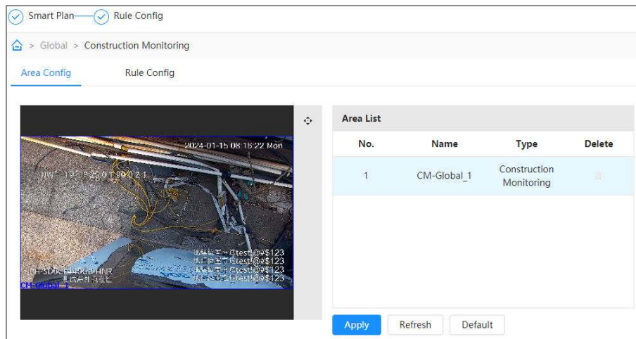
Figure 9-33 Area configuration
