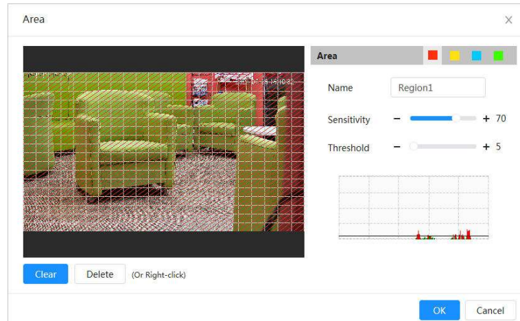
Figure 4-79 Area
