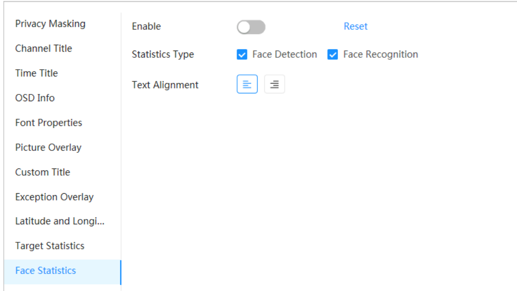
Figure 4-28 Face statistics
