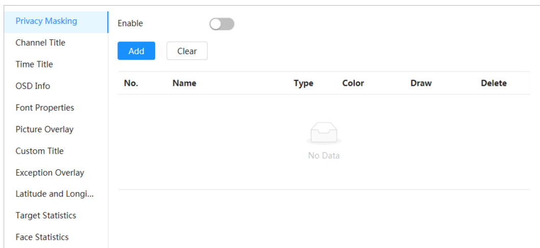
Figure 4-18 Privacy masking
