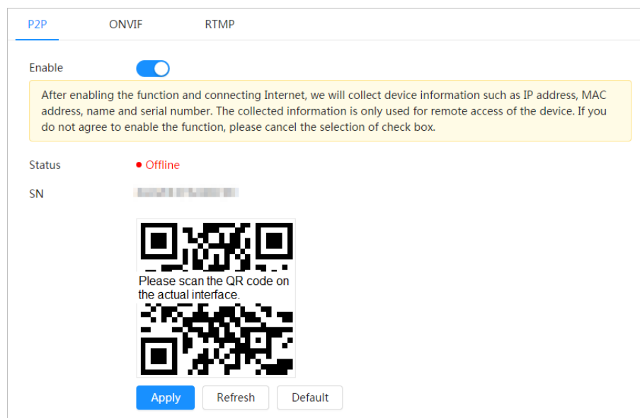
Figure 4-46 P2P
