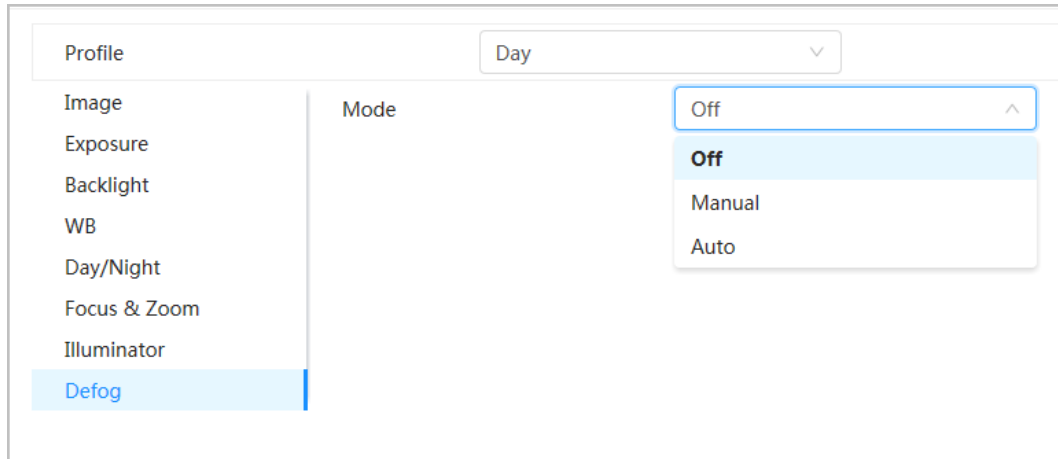
Figure 4-16 Defog
