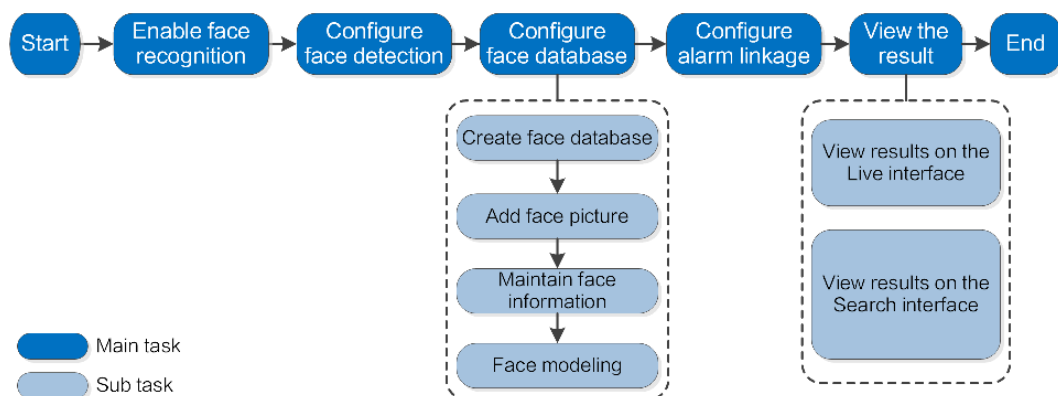
Figure 9-9 Face recognition flowchart
