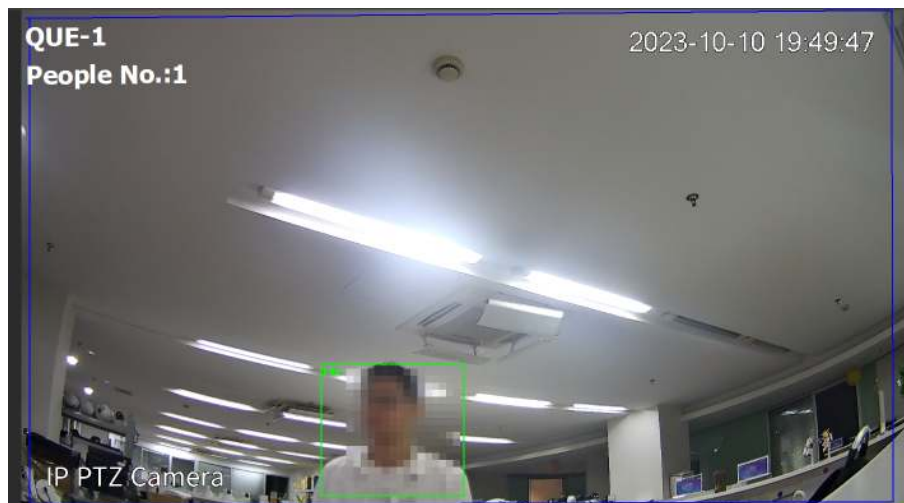
Figure 9-7 Queuing result
