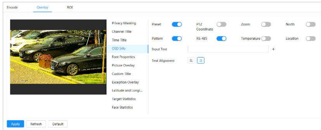
Figure 4-21 OSD info
