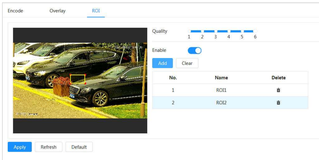
Figure 4-29 ROI
