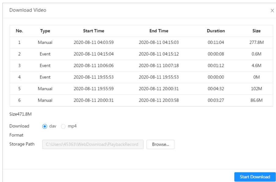
Figure 7-6 Downloading video
