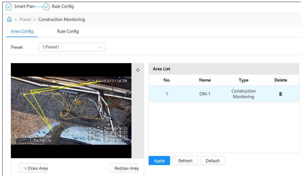
Figure 9-39 Area configuration
