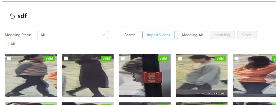
Figure 9-24 Import videos
