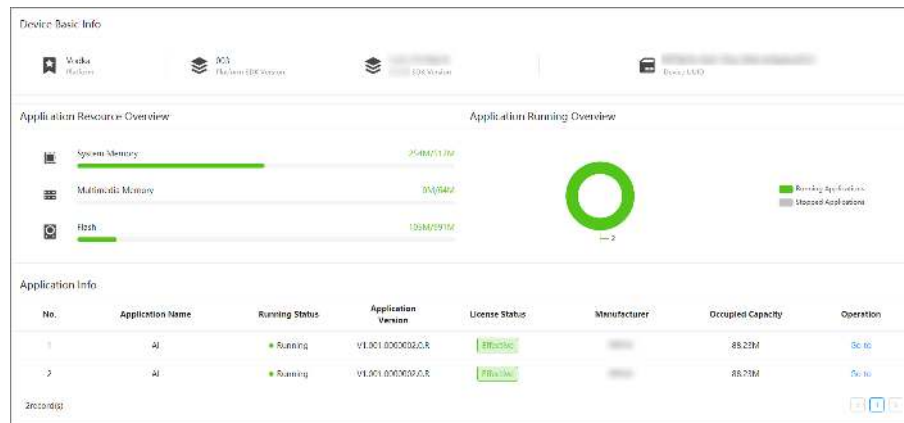
Figure 13-1 Application overview
