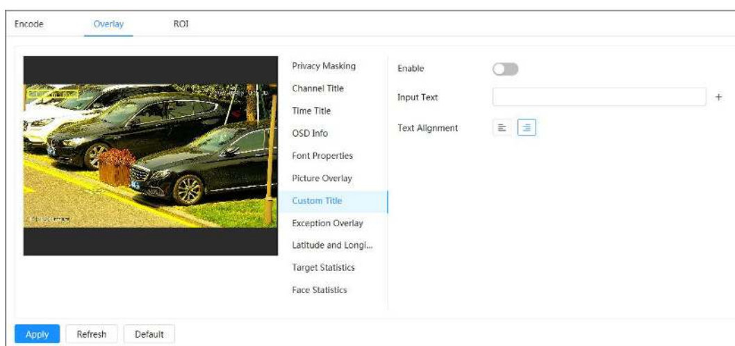
Figure 4-24 Custom title
