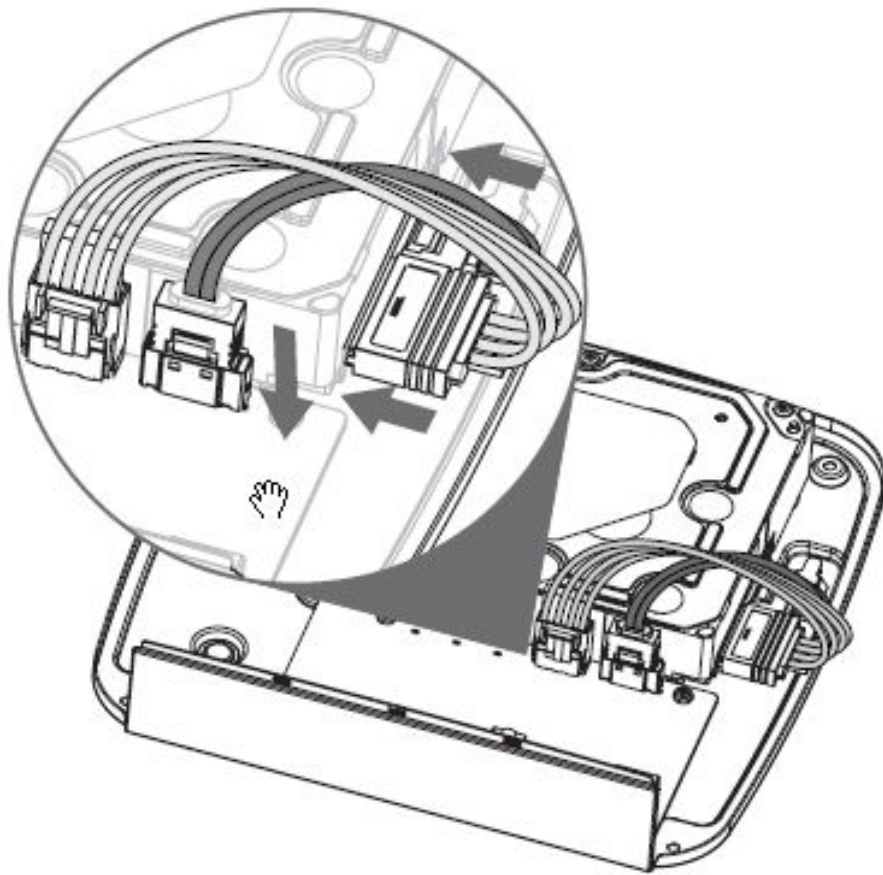
Figure 2-33 Connect cables
