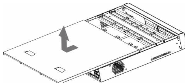
Figure 2-17 Remove cover
