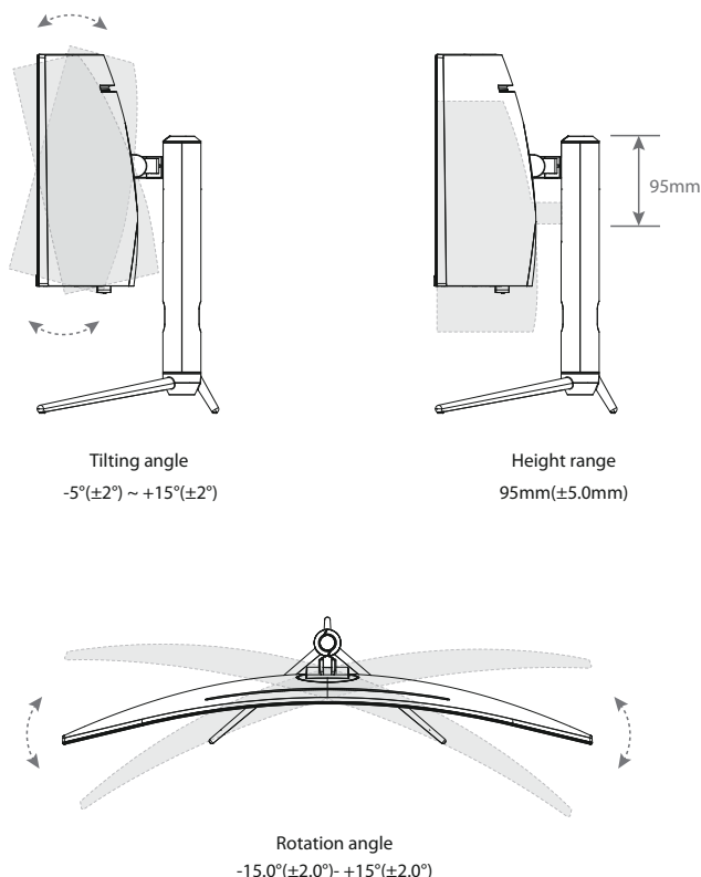
Figure 2-1 Angle Adjustment
