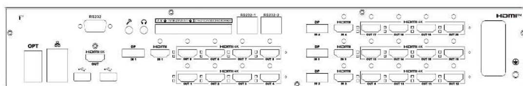
Figure 2-17 NVD2005DU-8I-8K-8H
