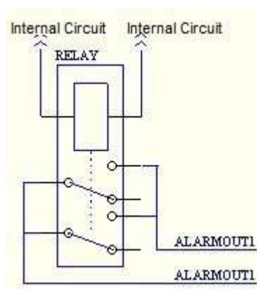
Figure 8-4 Diagram of alarm output port module
