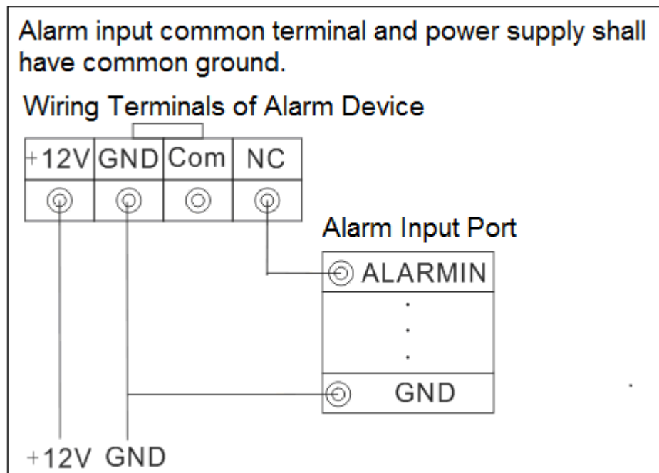
Figure 8-2 Diagram of alarm input
