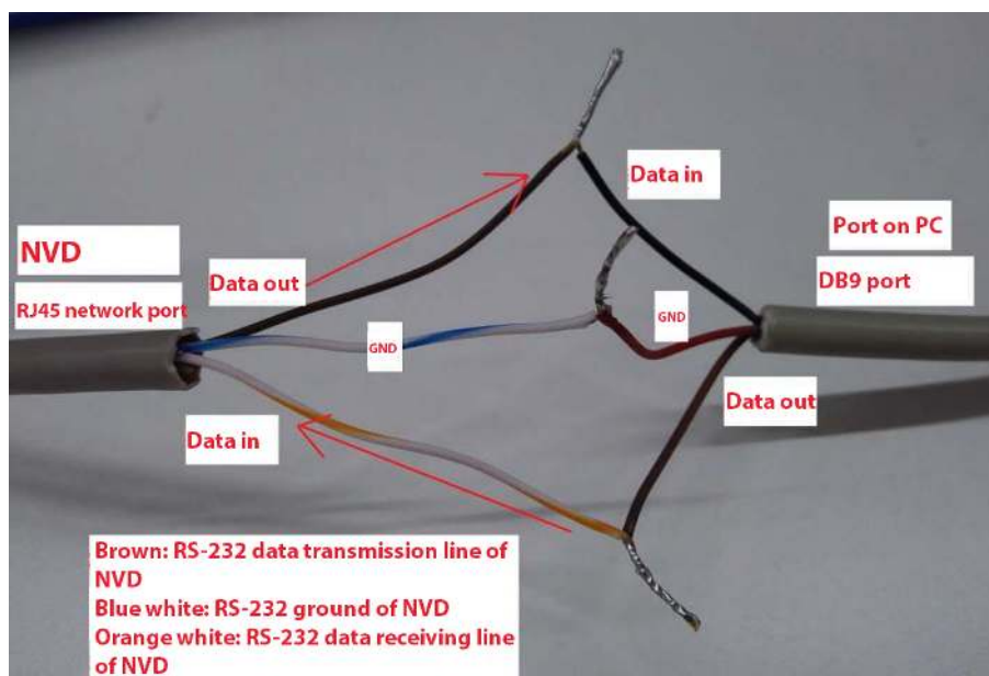
Figure 7-3 Wiring
