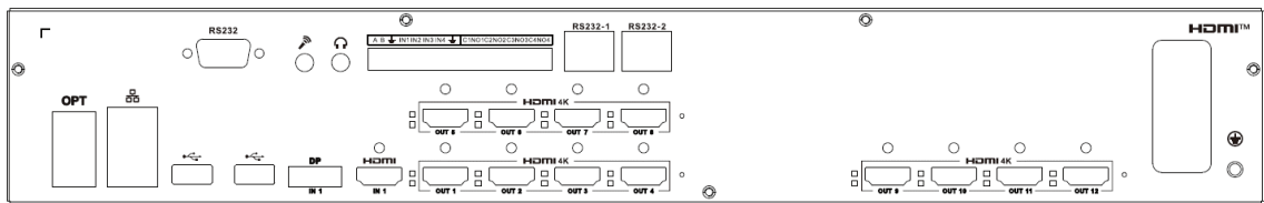
Figure 2-12 NVD0805DU-2I-8K rear panel
