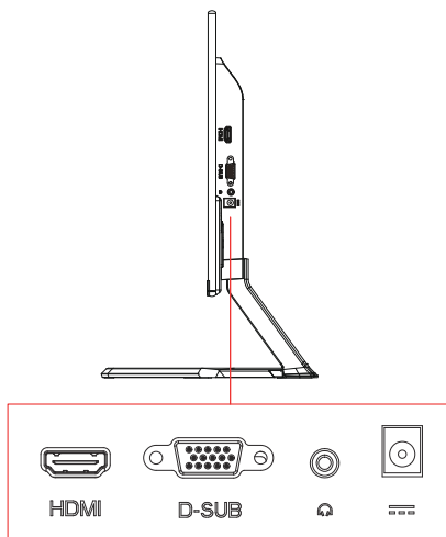
Figure 4-1 Input and output interface
