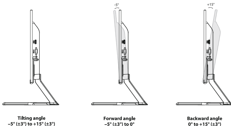
Figure 2-1 Angle Adjustment
