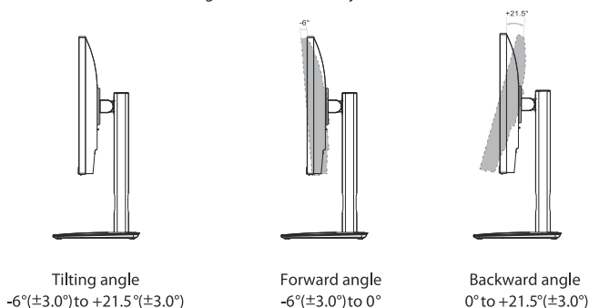
Figure 2-1 Monitor Adjustments
