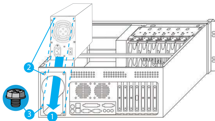
3.2.1.1. Power Supply (PSU) assembly
