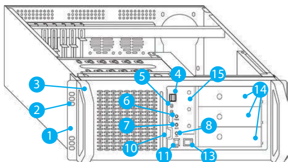
Figure 2.6.1.1 - SC01-4504-08B chassis
