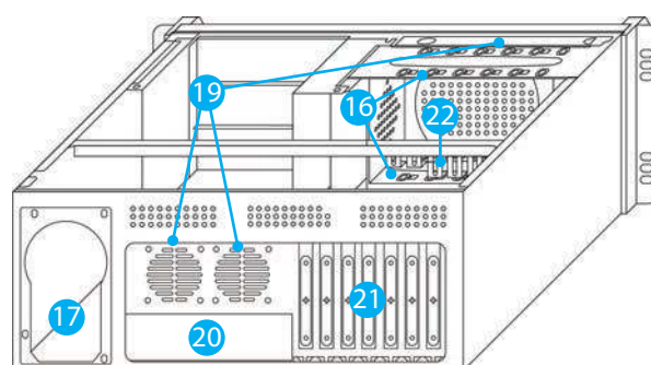
Figure 2.6.1.2 - SC01-4504-08B chassis
