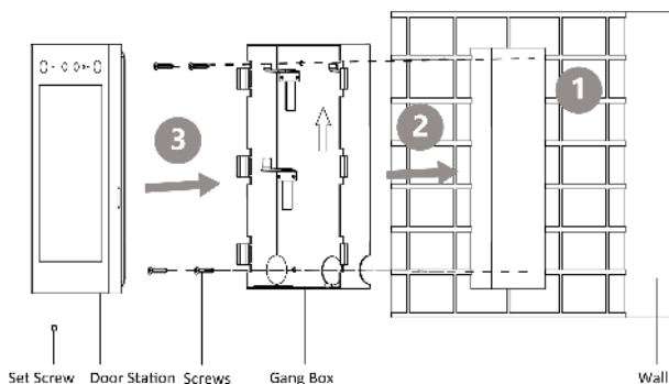
Figure 3-4 Flush Mounting
