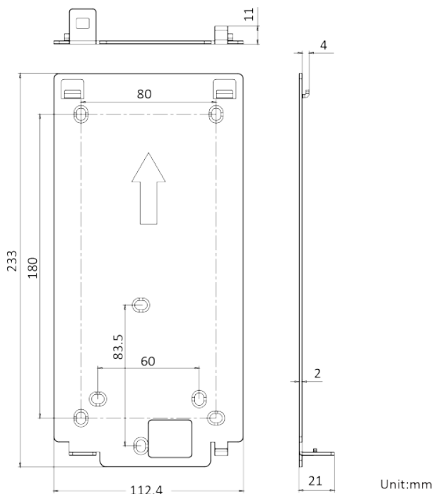
Figure 3-5 Mounting Plate
