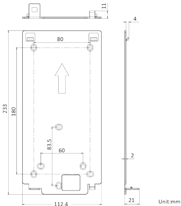
Figure 3-1 Mounting Plate
