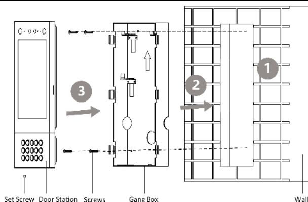
Figure 3-8 Flush Mounting
