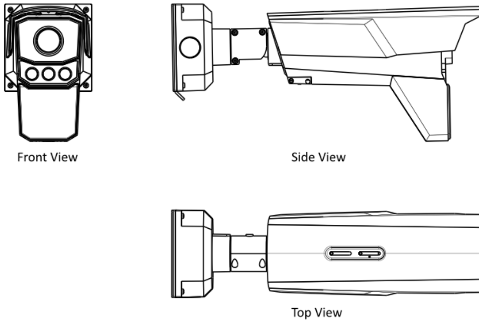
Figure 1-1 Appearance
