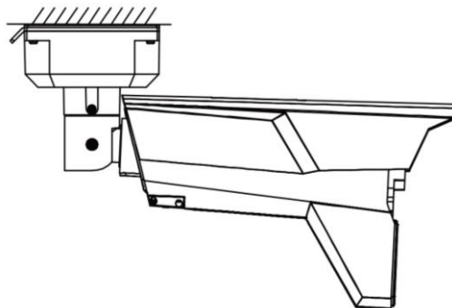
Figure 2-5 Fix Device onto Ceiling
