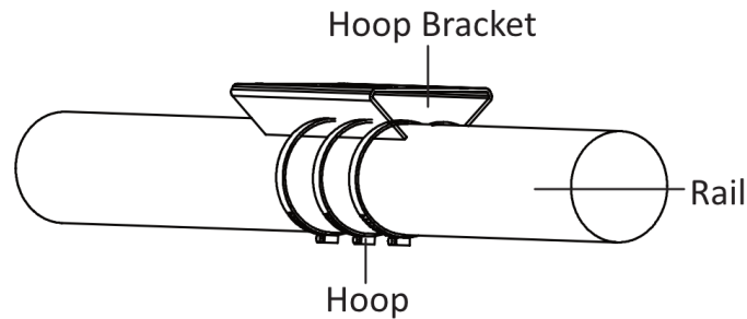
Figure 2-14 Install Hoops
