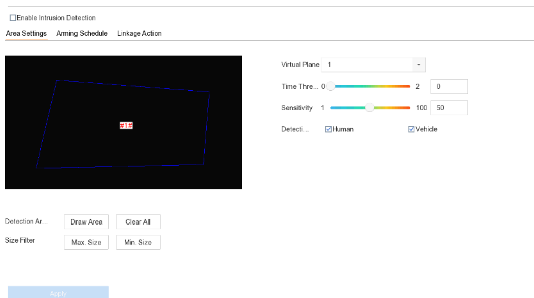
Figure 5-7 Intrusion Detection
