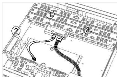
Figure 1-4 Connect Cable
