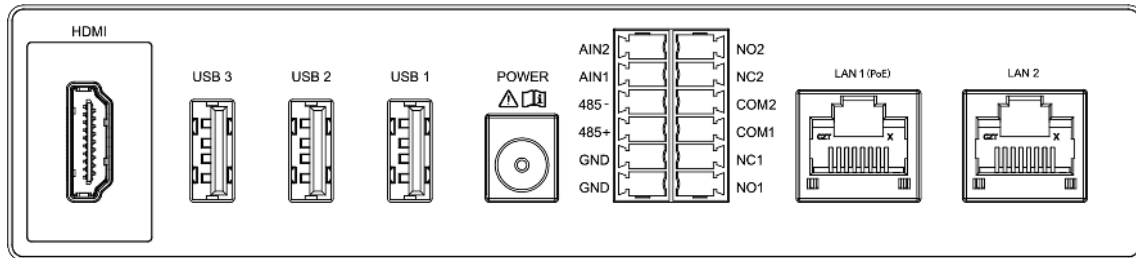
Figure 2-1 Terminal Description
