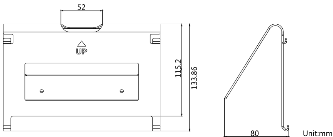
Figure 3-1 Table Bracket
