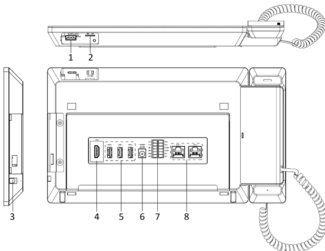
Figure 1-2 Top Panel and Rear Panel
