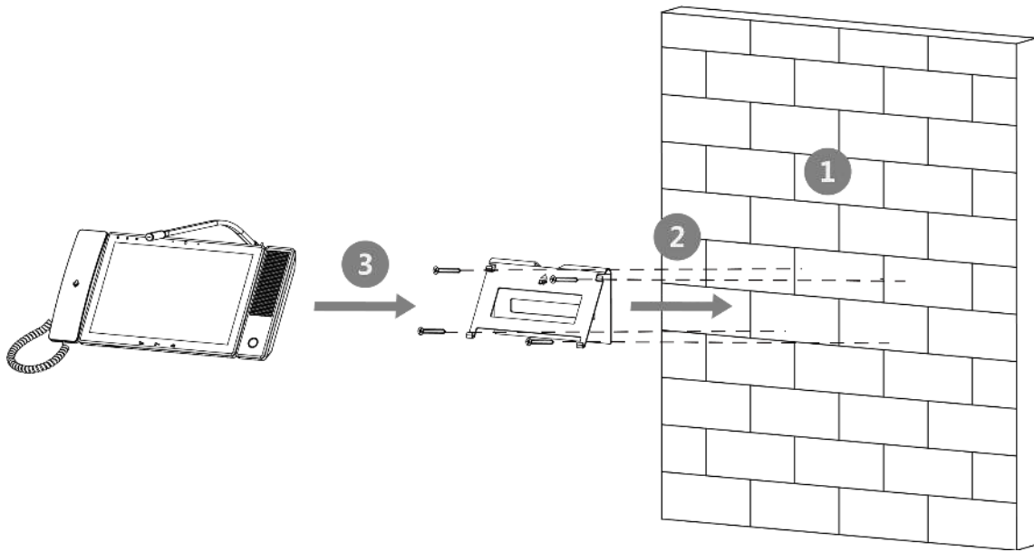
Figure 3-6 Wall Mounting
